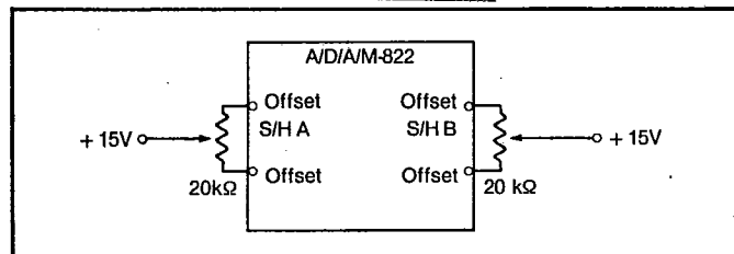
Figure 3. Offset Trimming Circuit.
