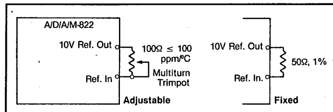
Figure 4. Gain Trimming Circuit.
