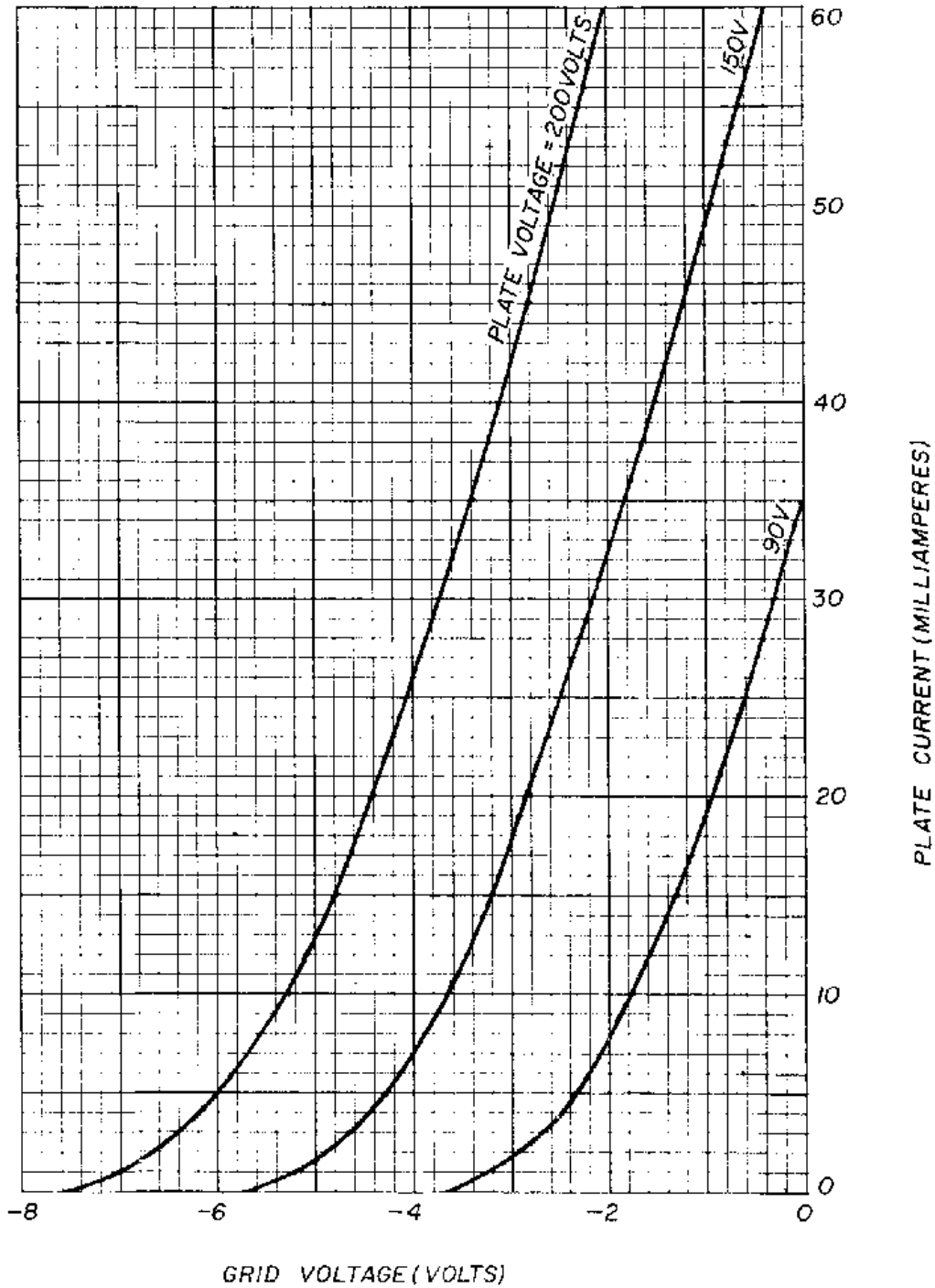
TRANSFER CHARACTERISTICS
