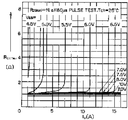
Typical Drain-Source on State Resistance vs. I_D
