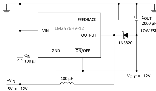
Figure 14. Negative Boost
