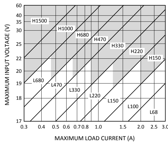
Figure 24. LM2576HV-15
