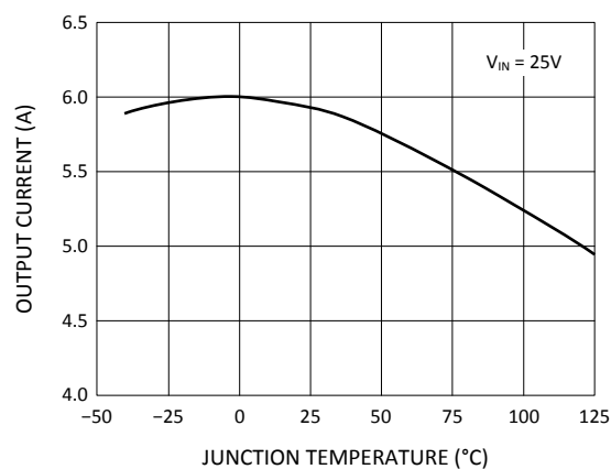
Figure 4. Current Limit
