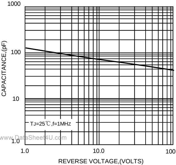
FIG.3-TYPICAL JUNCTION CAPACITANCE
