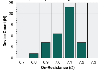
Typical On-Resistance Distribution (N=50, I_F=0.5\text{mA} , I_L=75\text{mA} )
