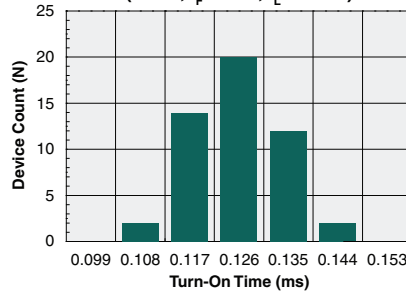
Typical Turn-On Time (N=50, I_F=2\text{mA} , I_L=75\text{mA} )
