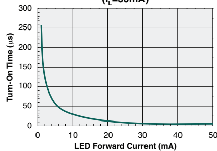
Typical Turn-On Time vs. LED Forward Current ( I_L=50\text{mA} )
