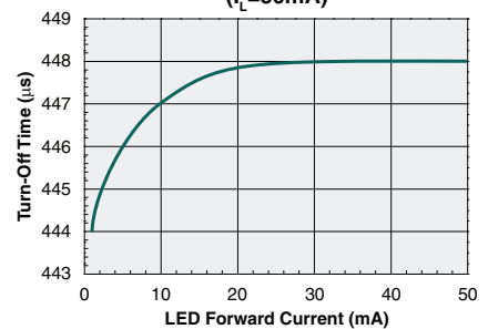
Typical Turn-Off Time vs. LED Forward Current ( I_L=50\text{mA} )
