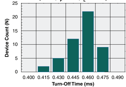
Typical Turn-Off Time (N=50, I_F=2\text{mA} , I_L=75\text{mA} )
