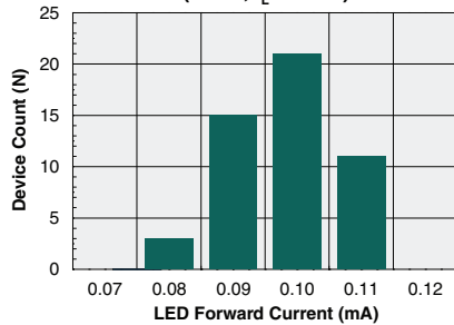
Typical I_F for Switch Operation (N=50, I_L=75\text{mA} )
