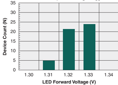
Typical LED Forward Voltage Drop (N=50, I_F=10\text{mA} , I_L=1A_{DC} )
