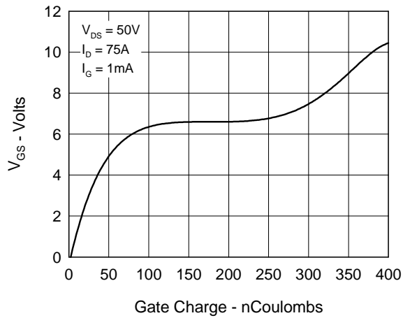
www.DataSheet4U.com Fig.7 Gate Charge Characteristic Curve
