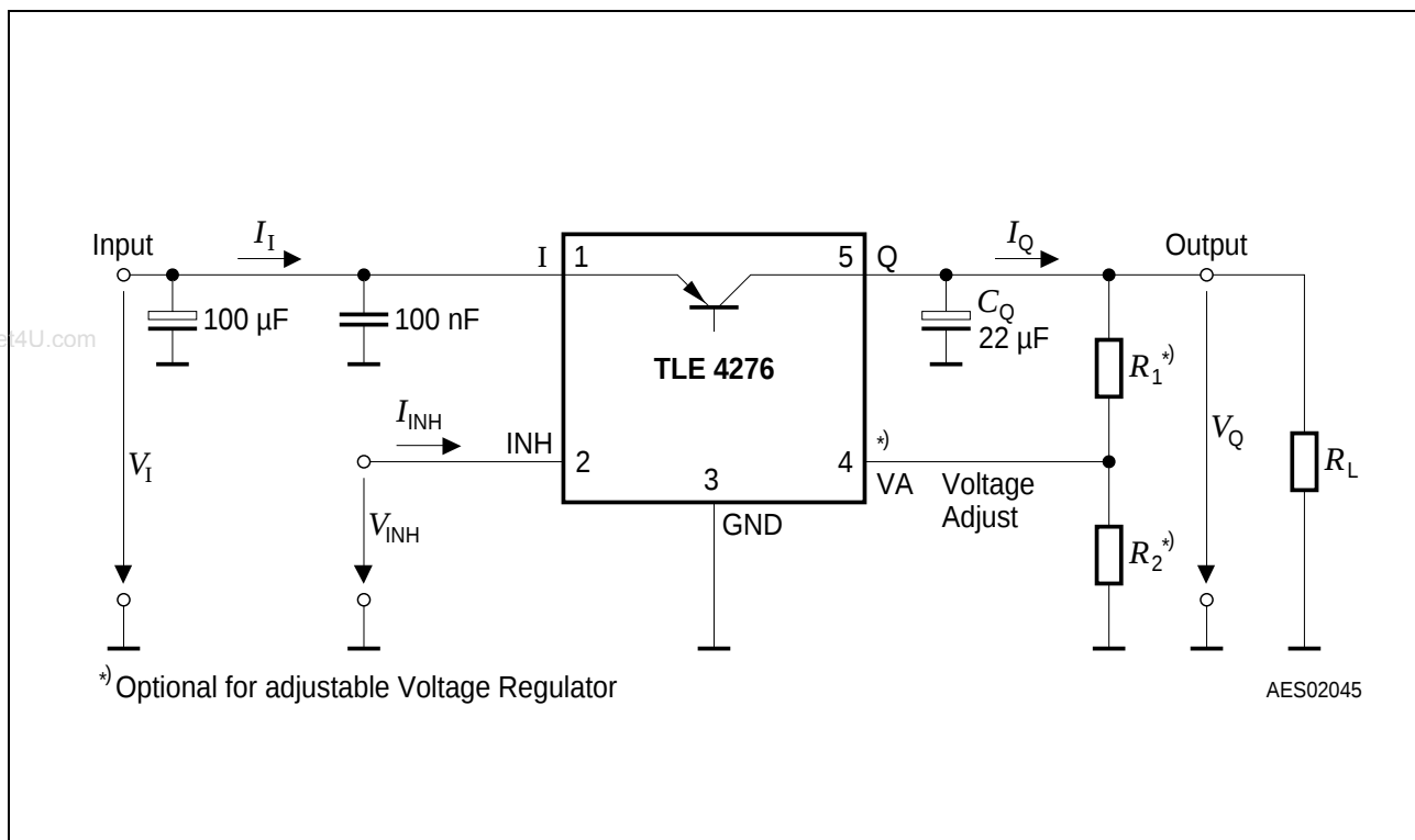
Figure 3 Measuring Circuit
