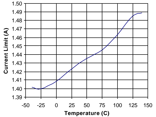
Figure 15 - Typical Current Limit vs. Temperature ( V_{IN}=5.5\text{V} )
