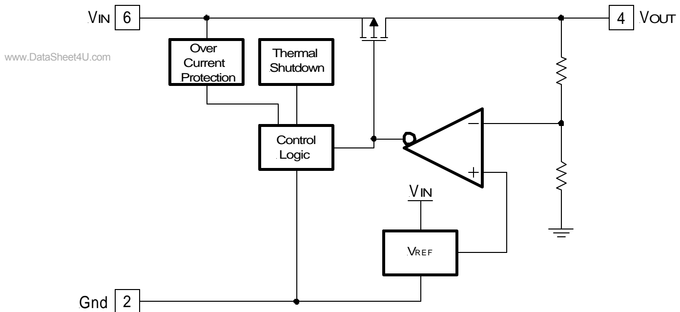
Figure 2 - Simplified block diagram of the IRU1502-33.
