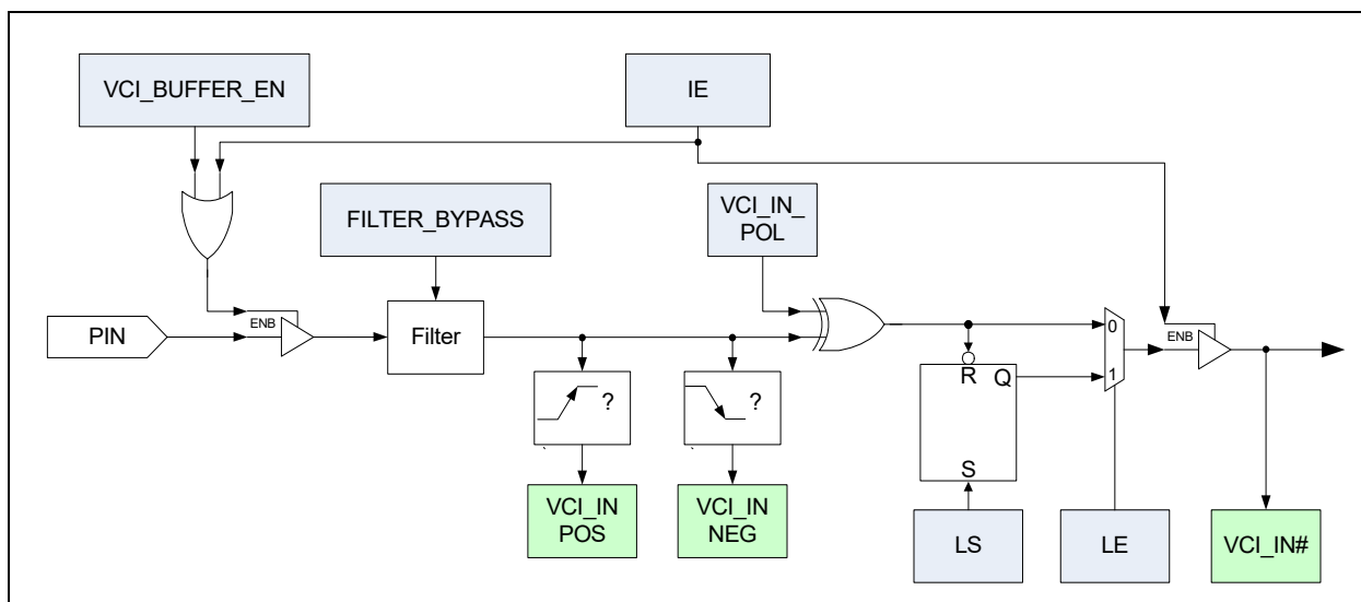
FIGURE 47-3: VBAT-POWERED CONTROL INTERFACE BLOCK DIAGRAM
