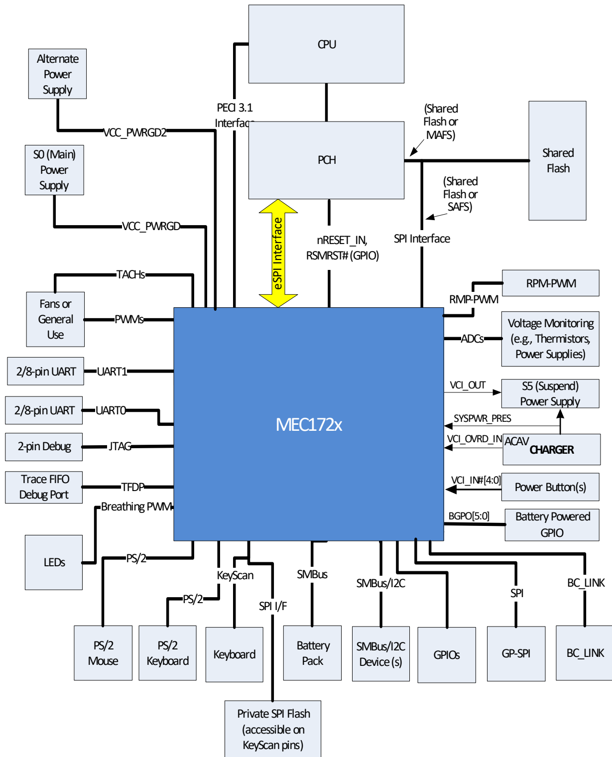
FIGURE 1-1: BLOCK DIAGRAM
