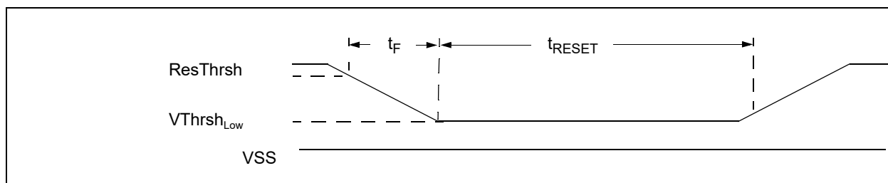
FIGURE 57-2: VTR RESET AND POWER-DOWN
