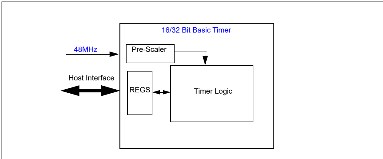
FIGURE 21-2: BLOCK DIAGRAM
