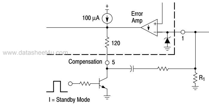
Figure 16. Low Power Standby Circuit
