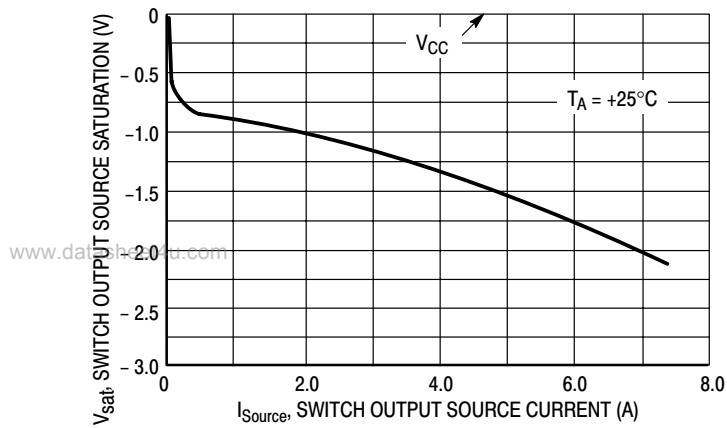
Figure 8. Switch Output Source Saturation versus Source Current
