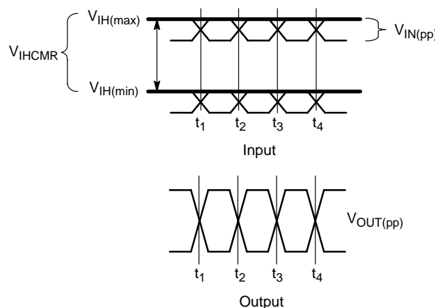
Figure 11. V_{IH} Common Mode Range, V_{IHCMR}
