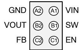
Figure 3. WLCSP (Bottom View)
