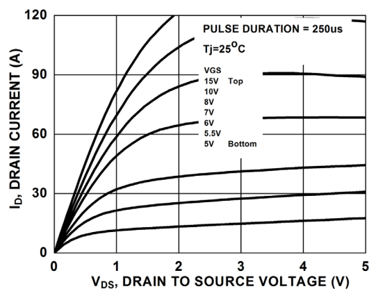
Figure 9. Saturation Characteristics
