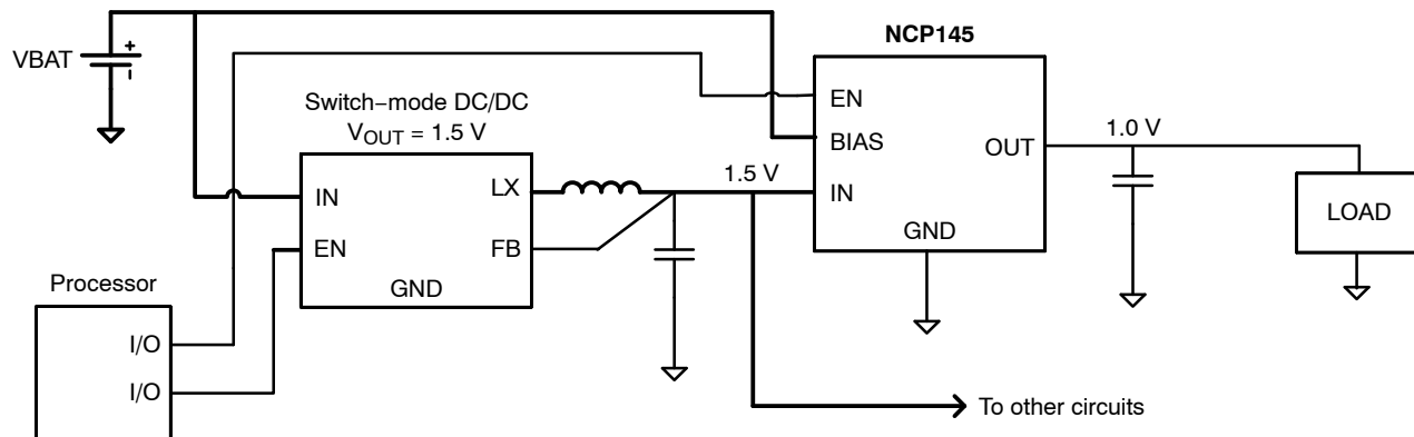
Figure 17. Typical Application: Low-Voltage DC/DC Post-Regulator with ON/OFF Functionality
