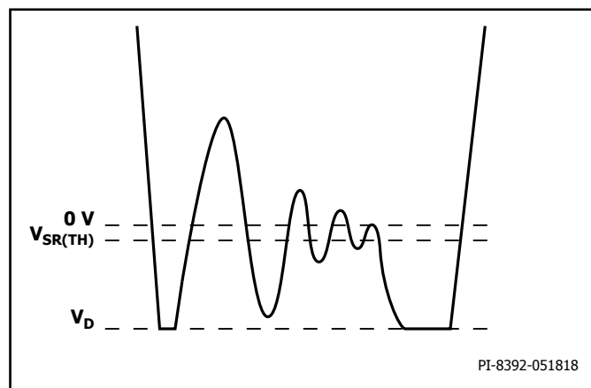
Figure 7. Unacceptable FORWARD Pin Waveform After Handshake with SR Switch Conduction During Flyback Cycle.
