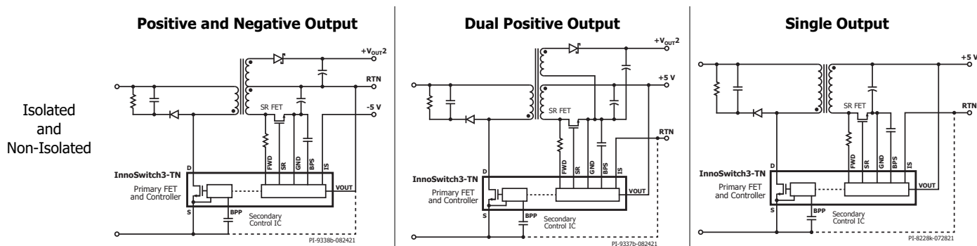
Figure 1. Power Supply Configuration Examples using InnoSwitch3-TN.
