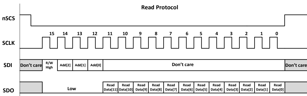
Figure 42. Read Protocol
