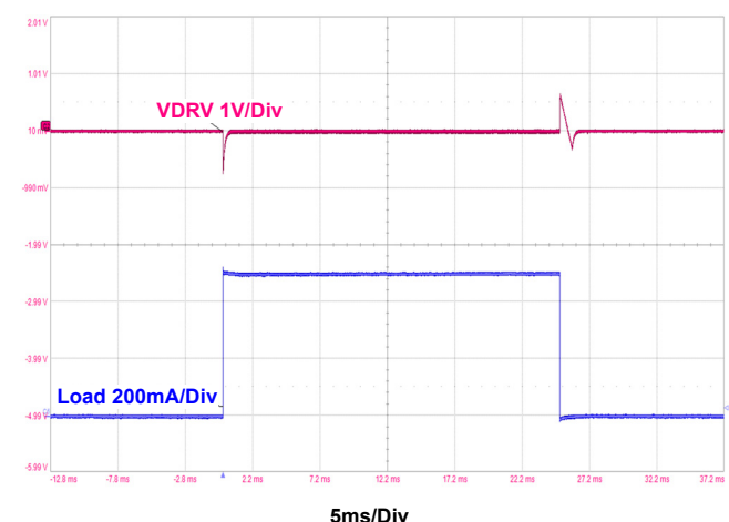
Figure 18. Buck-Boost Regulator 500mA Load Transient, VM = 48V
