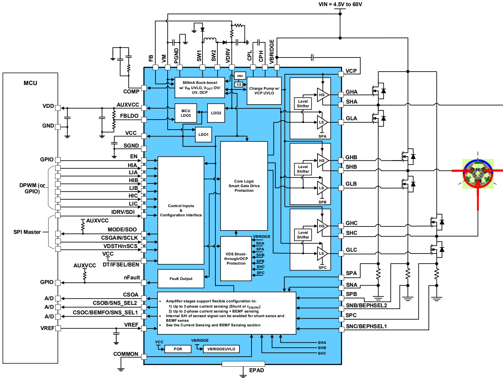
Figure 1. Typical Application Diagram
