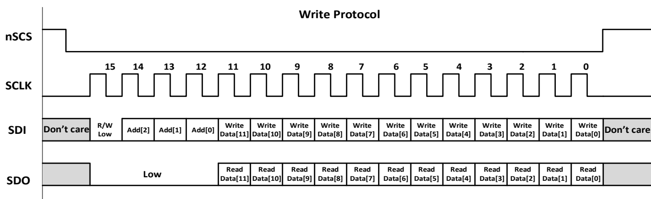
Figure 41. Write Protocol
