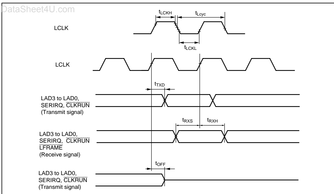
Figure 28.30 Host Interface (LPC) Timing
