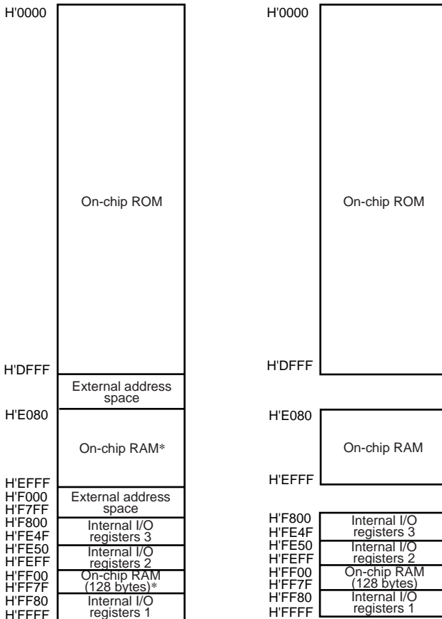
Figure 3.2 Address Map for H8S/2140B and H8S/2160B (2)
