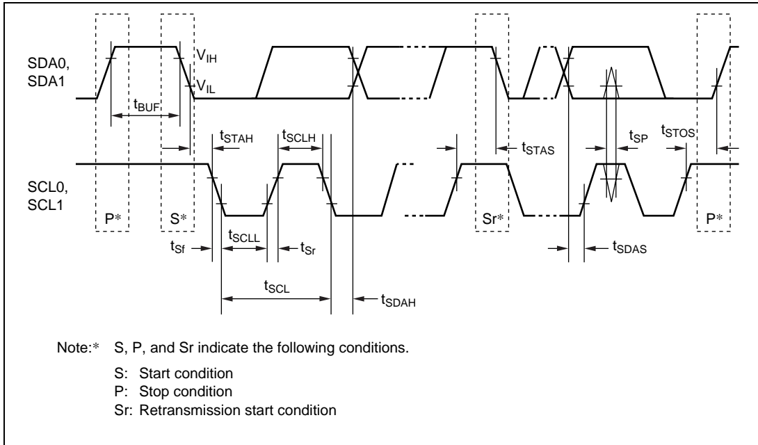
Figure 28.29 I 2 C Bus Interface Input/Output Timing
