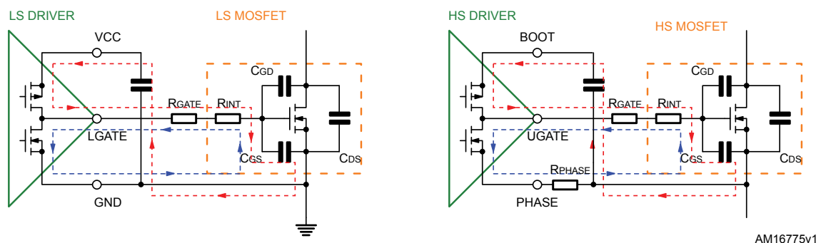
Figure 11. Driver- turn-on and turn-off paths
