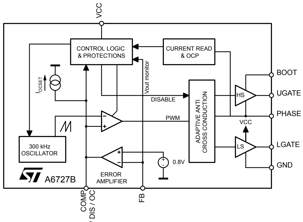
Figure 2. Block diagram
