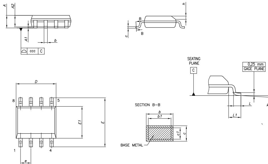
Figure 13. SO-8 package dimensions
