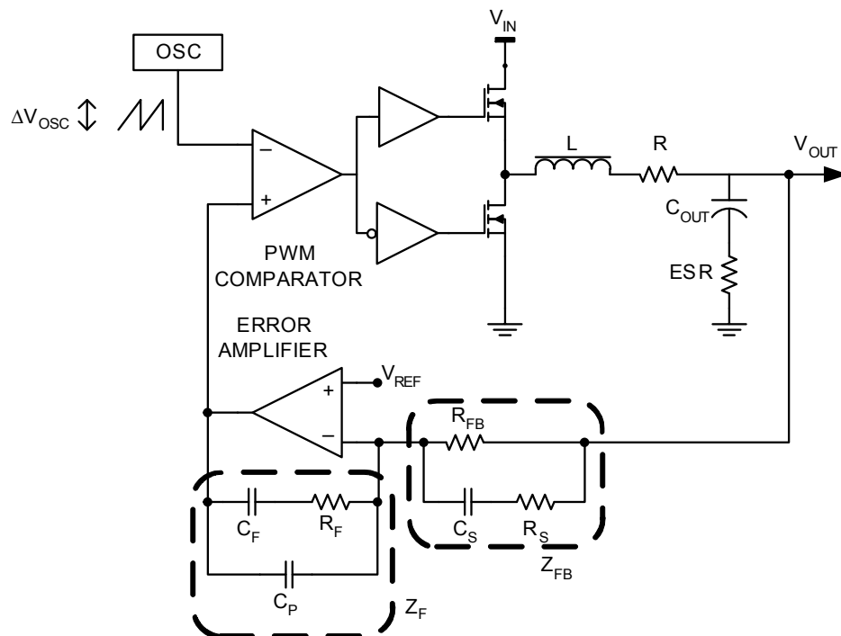
Figure 8. PWM control loop
