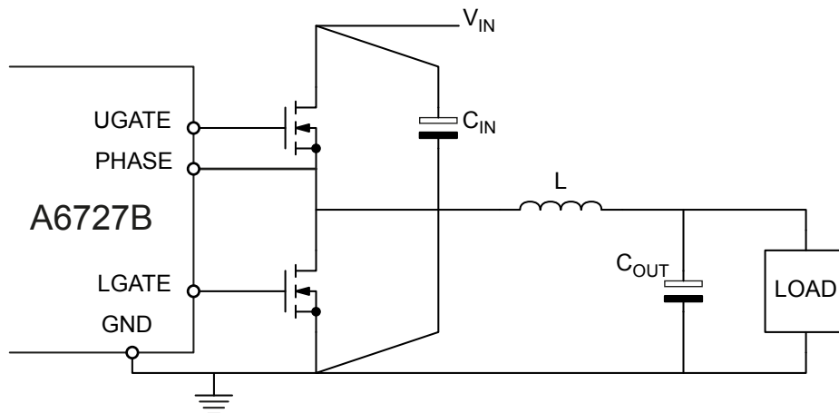
Figure 10. Power connections (heavy lines)
