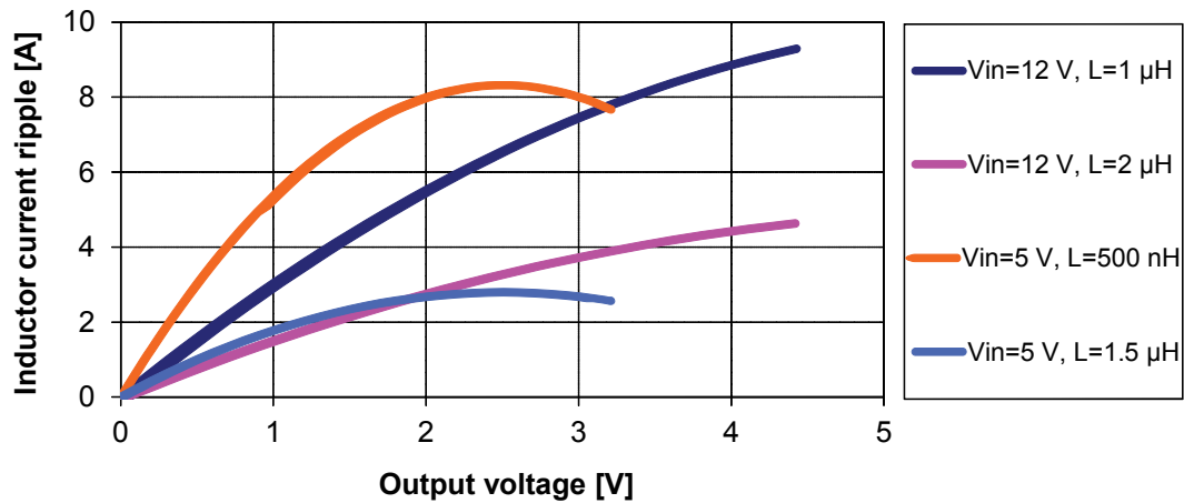
Figure 12. Inductor current ripple vs. output voltage
