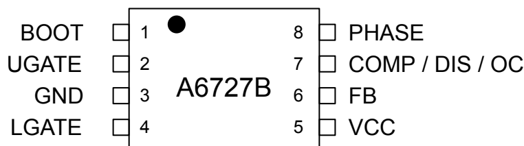
Figure 3. Pin connection (top view)
