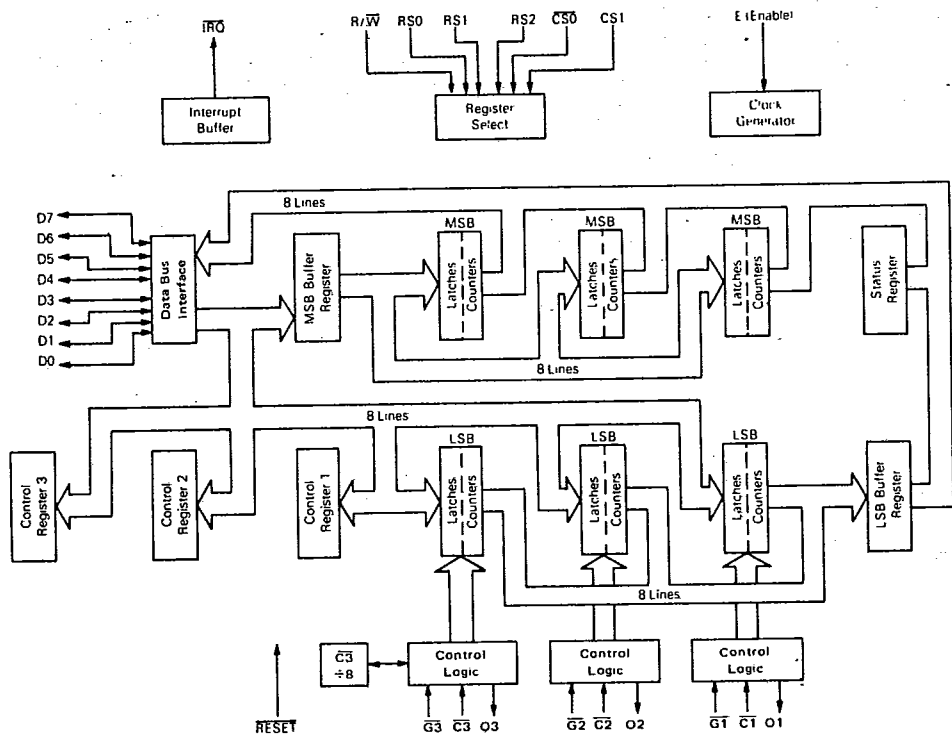
FIGURE 2 — BLOCK DIAGRAM
