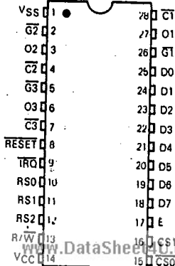
FIGURE 1 - PIN ASSIGNMENT
