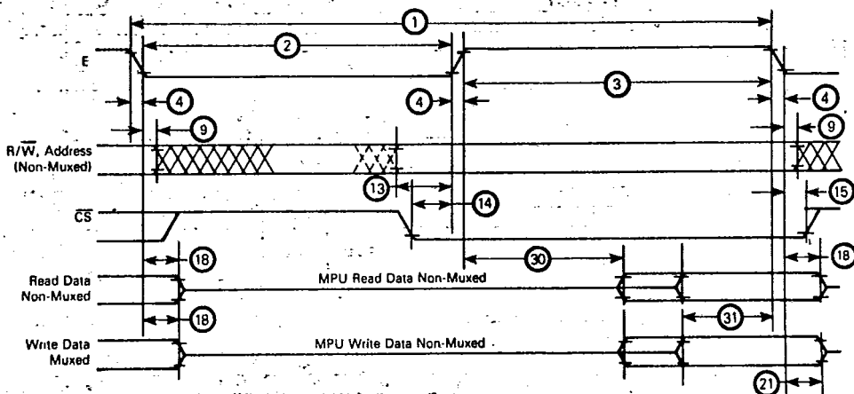
FIGURE 3 — BUS TIMING
