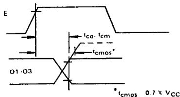
FIGURE 7 - OUTPUT DELAY
