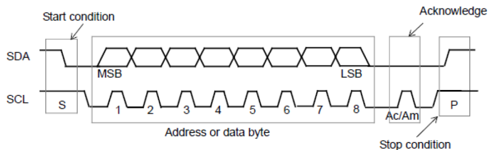
Figure 10. Data transfer protocol
