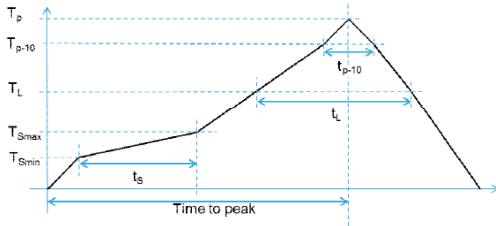
Figure 34. Solder profile
