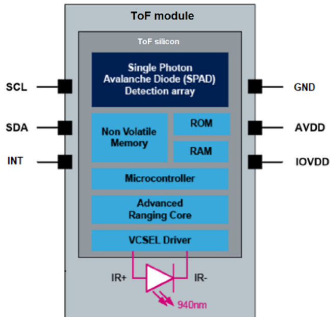
Figure 3. VL53L8CX block diagram
