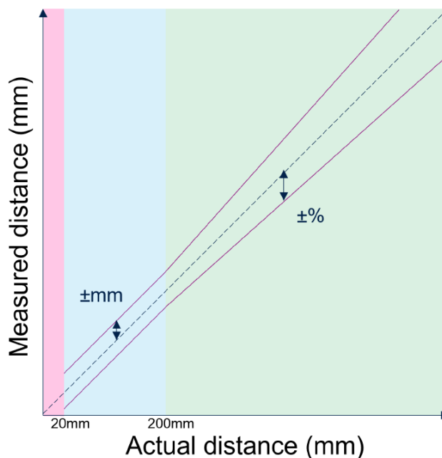
Figure 25. Range accuracy vs distance
