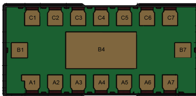
Figure 4. VL53L8CX pinout (bottom view)
