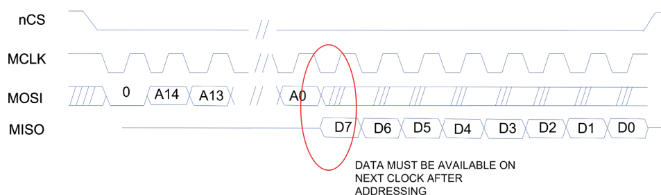
Figure 19. SPI read timing
