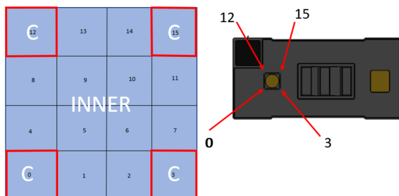
Figure 21. Zone mapping in 4x4 mode
