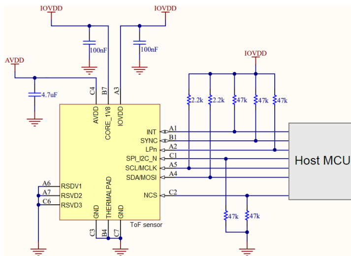
Figure 5. Typical application schematic for I 2 C
