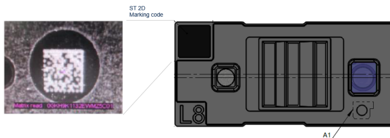
Figure 32. 2D marking product code
