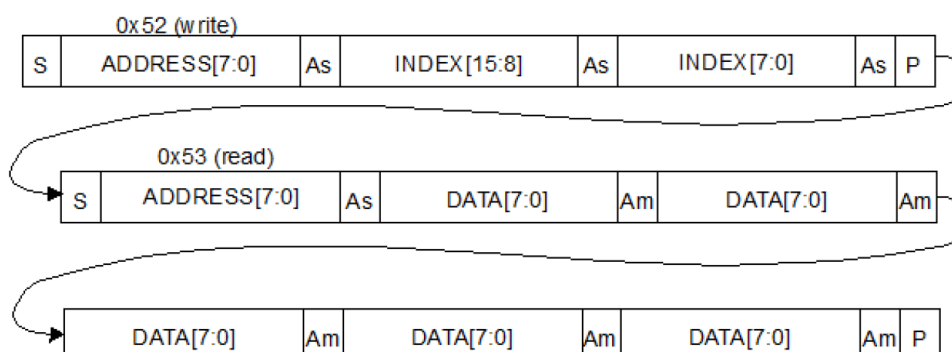
Figure 15. VL53L8CX data format (sequential read)
