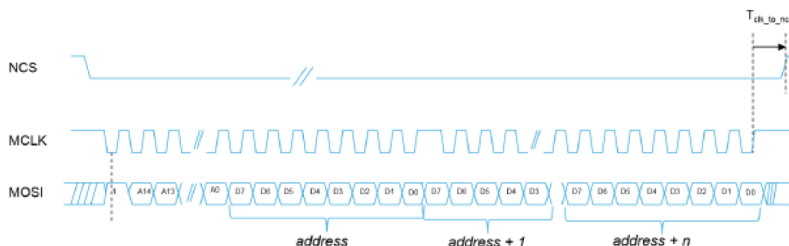
Figure 18. SPI auto-increment write sequence
