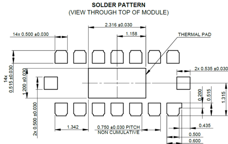
Figure 35. Recommended solder pattern
