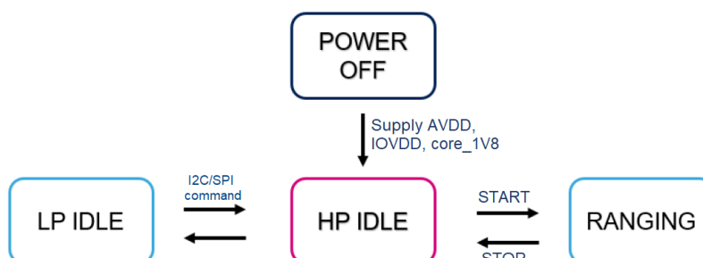
Figure 8. Power state machine
