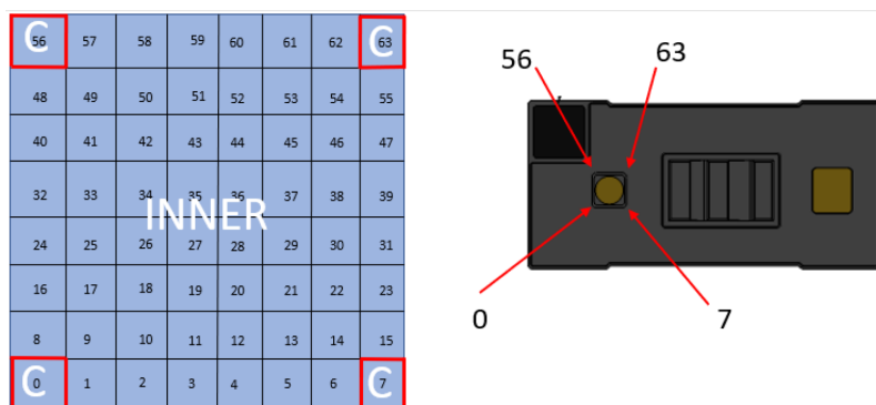
Figure 22. Zone mapping in 8x8 mode
