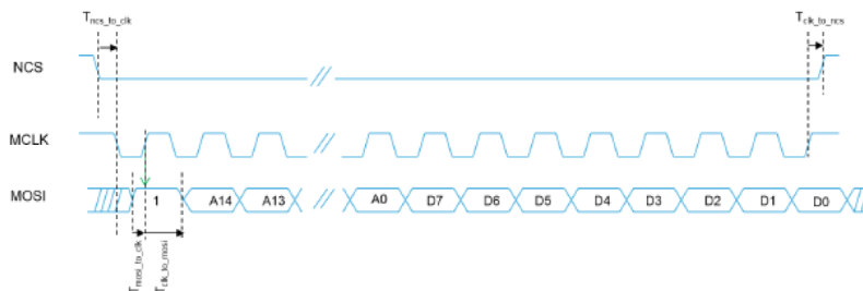
Figure 17. SPI writing timing sequence
