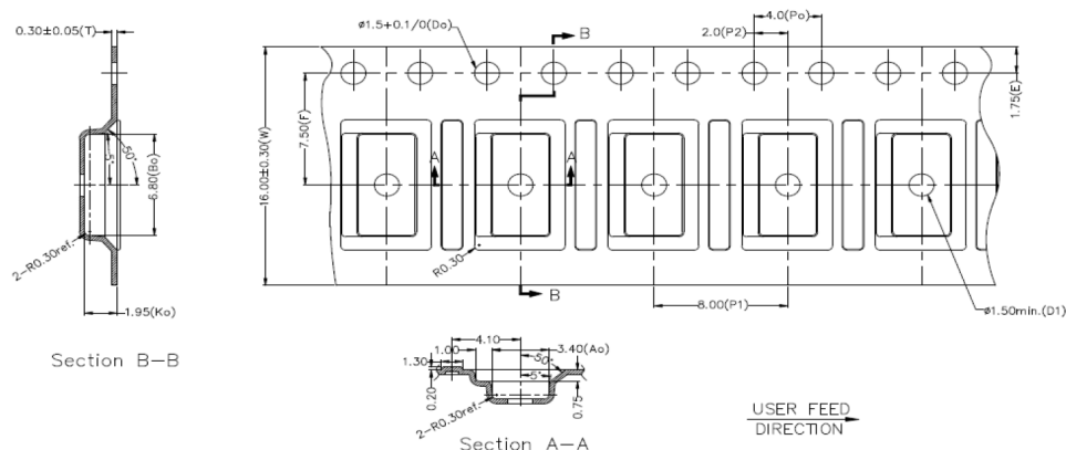
Figure 33. VL53L8CX tape and reel packaging drawing
