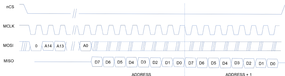
Figure 20. SPI auto-increment read sequence
