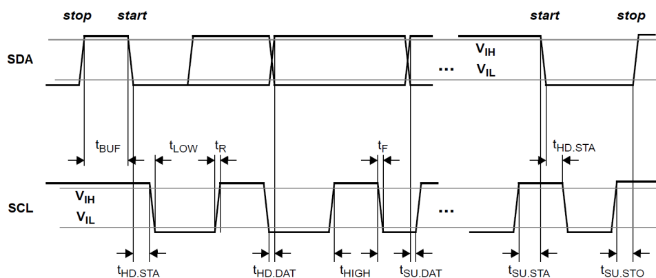
Figure 16. I 2 C timing characteristics
