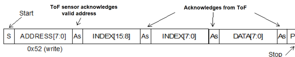
Figure 12. VL53L8CX data format (write)
