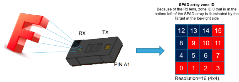
Figure 23. Effective orientation
