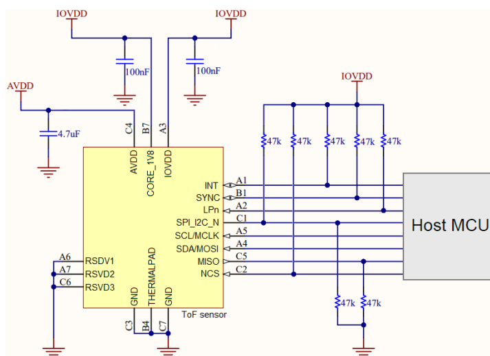
Figure 6. Typical application schematic for SPI
