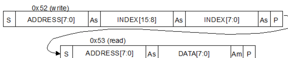
Figure 13. VL53L8CX data format (read)
