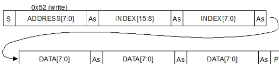
Figure 14. VL53L8CX data format (sequential write)
