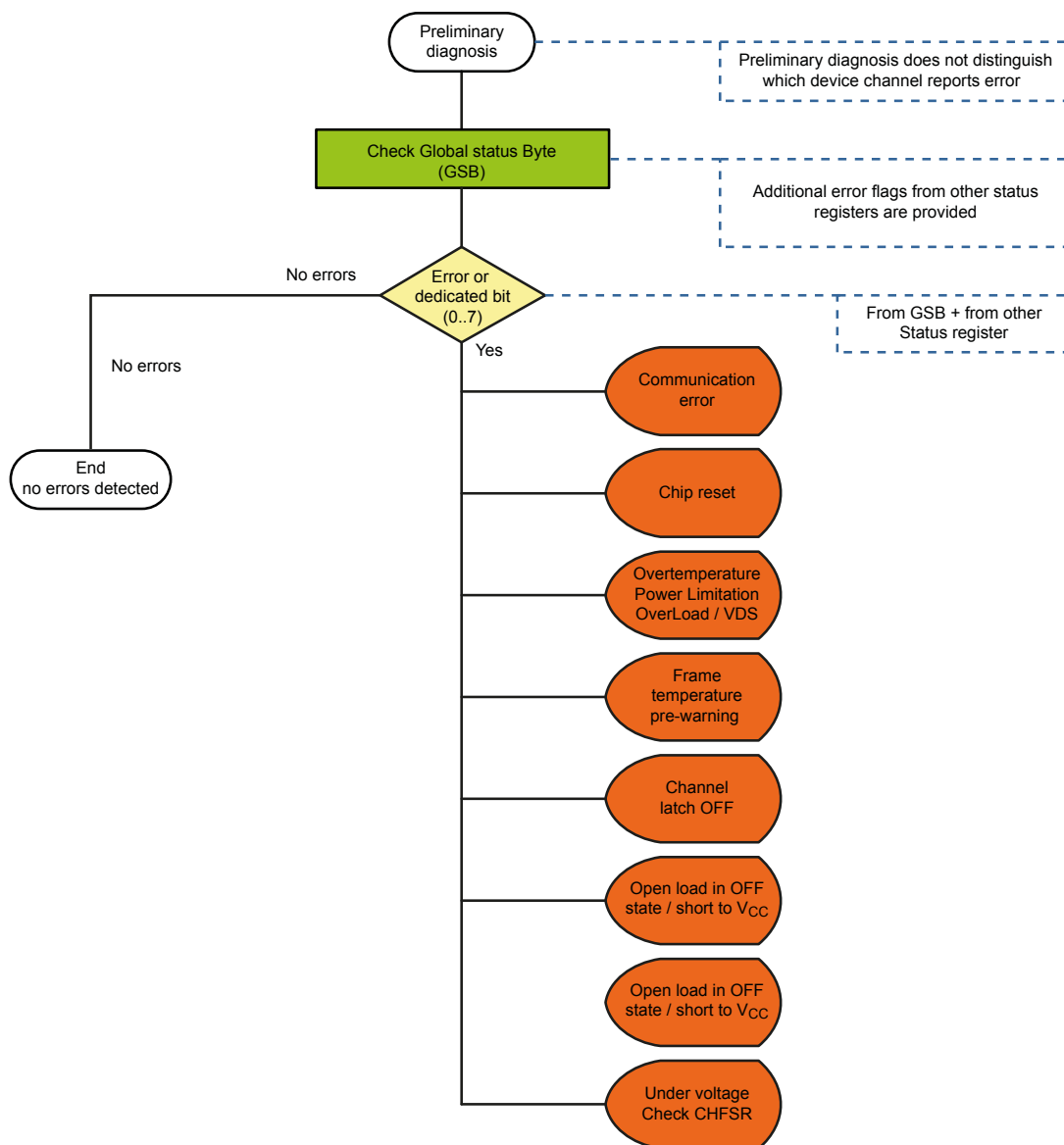
Figure 23. Status registers
