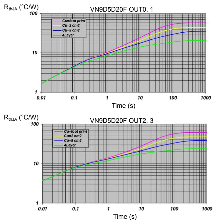
Figure 49. QFN 6x6 thermal impedance junction ambient
