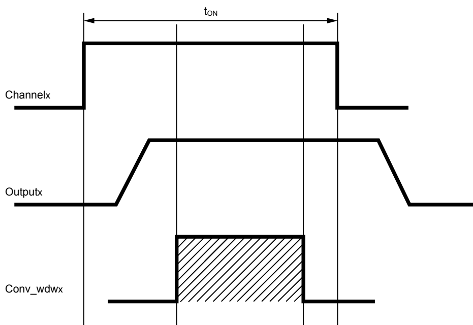
Figure 18. Conversion window generation
