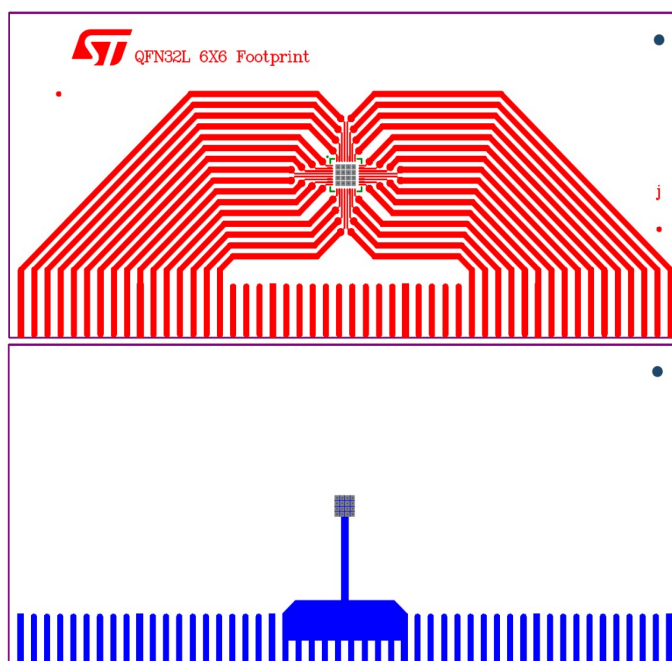
Figure 44. QFN 6x6 PCB footprint
