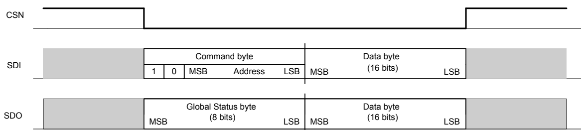
Figure 10. SPI read and clear operation
