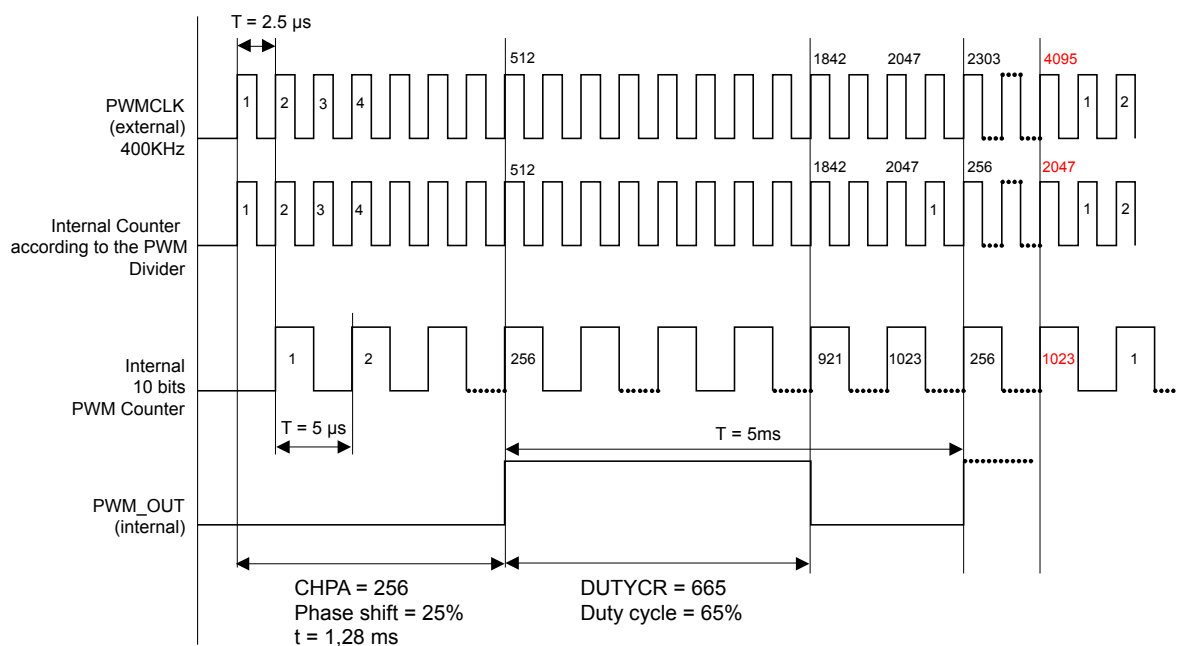
Figure 12. Resulting waveform 1
