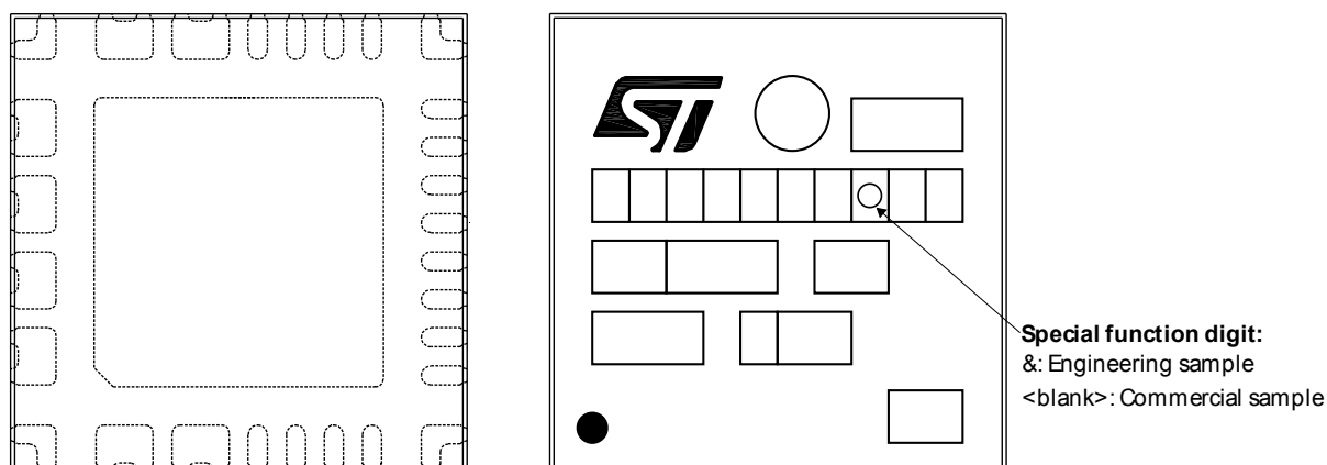
Figure 43. QFN 6x6 marking information
