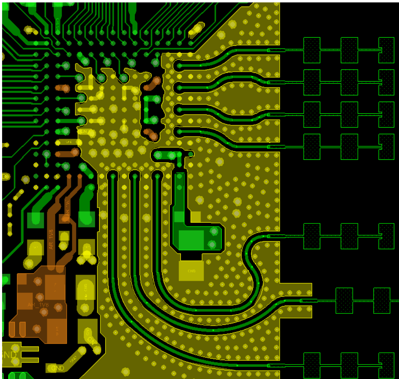
Figure 11-5. Top Layer Routing Closeup
