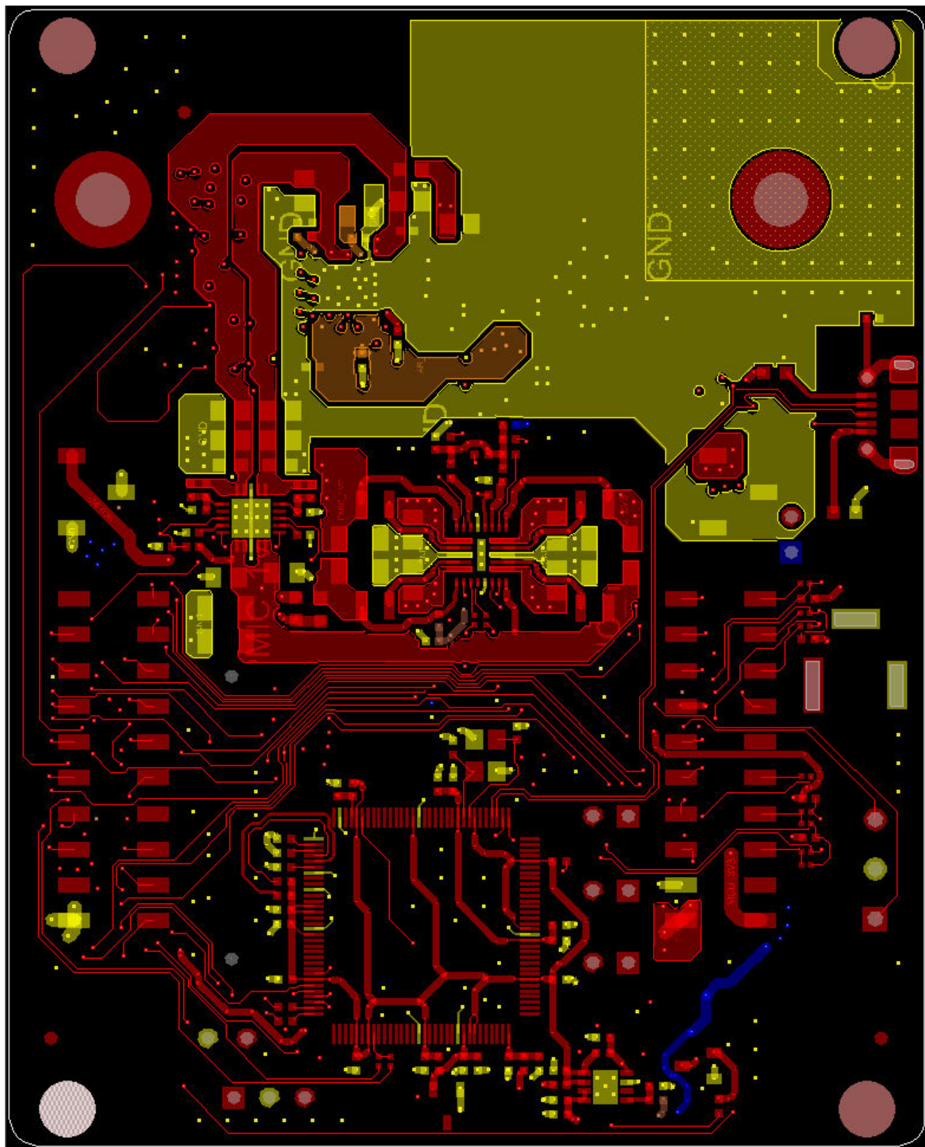
Figure 11-6. Bottom Layer Routing
