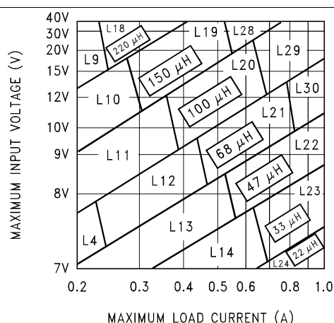
Figure 28. LM2595 5-V
