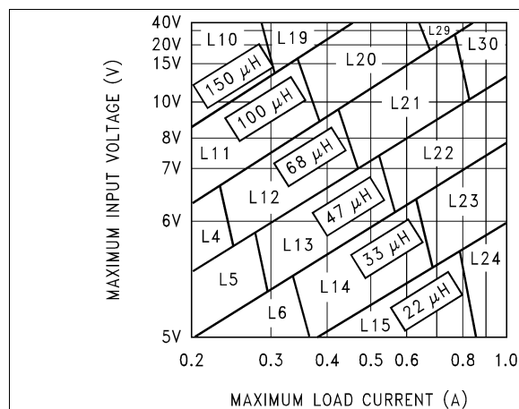
Figure 27. LM2595 3.3-V
