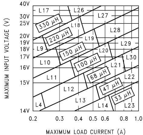
Figure 29. LM2595 12-V
