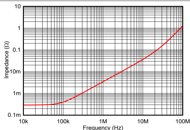
Figure 7-17. Closed-Loop Output Impedance vs Frequency
