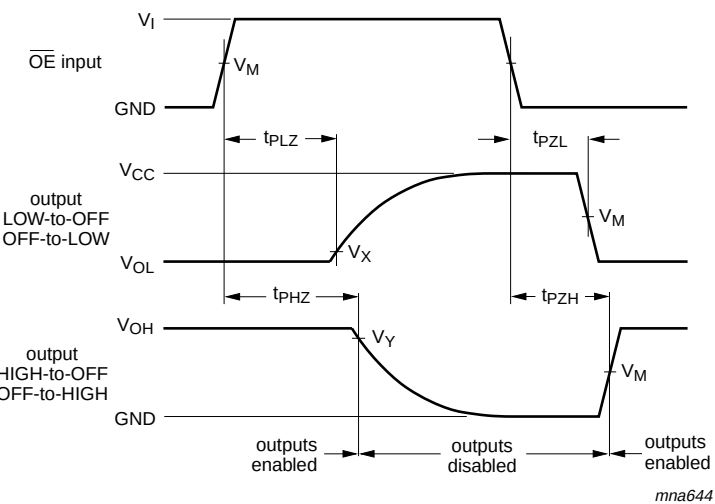
Measurement points are given in Table 8 . VOL and VOH are the typical output voltage drops that occur with the output load.
